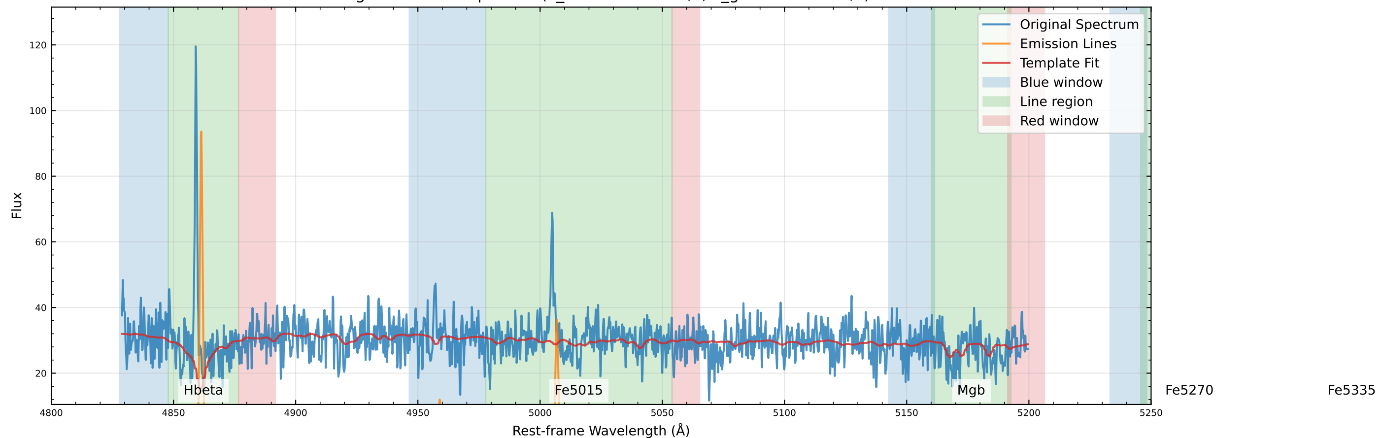
Original Data Comparison (v_star=-106.8 km/s, v_gas=-129.4 km/s)
