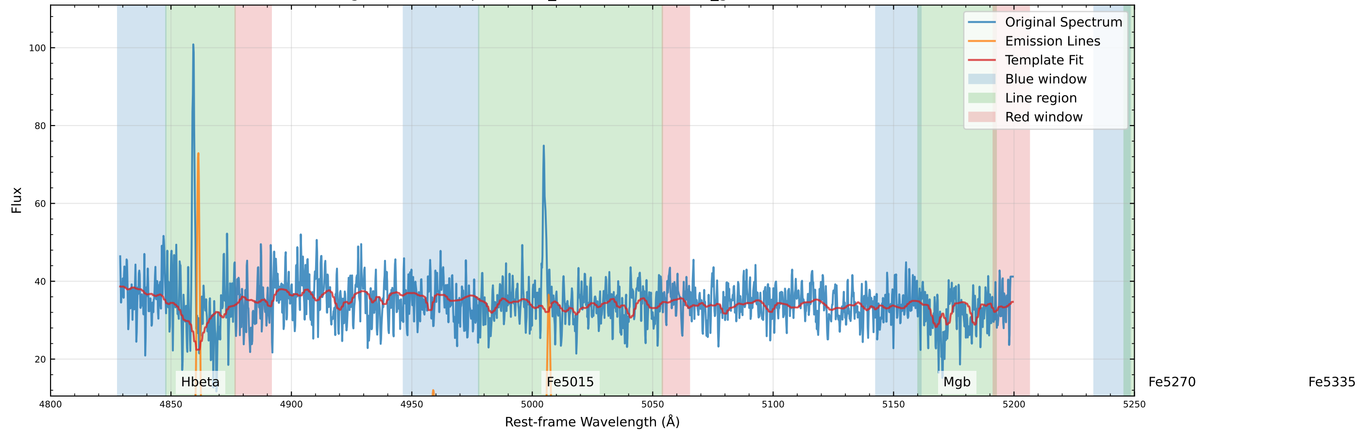
Original Data Comparison (v_star=-122.9 km/s, v_gas=-122.3 km/s)
