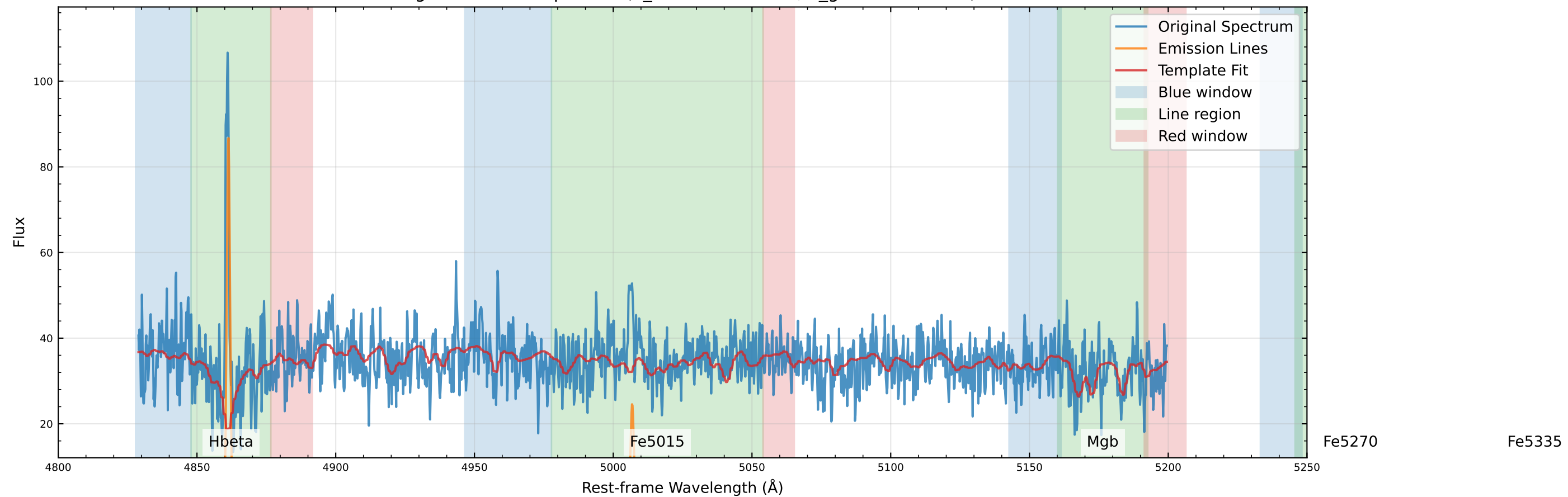
Original Data Comparison (v_star=-37.5 km/s, v_gas=-27.0 km/s)
