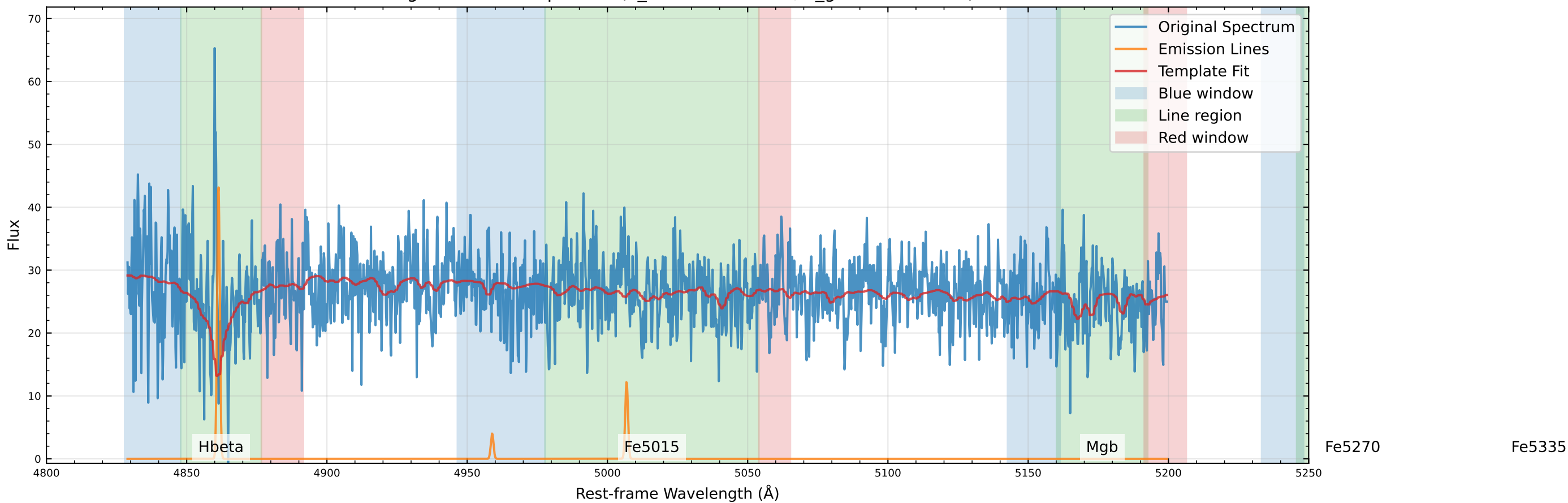
Original Data Comparison (v_star=-84.0 km/s, v_gas=-74.9 km/s)
