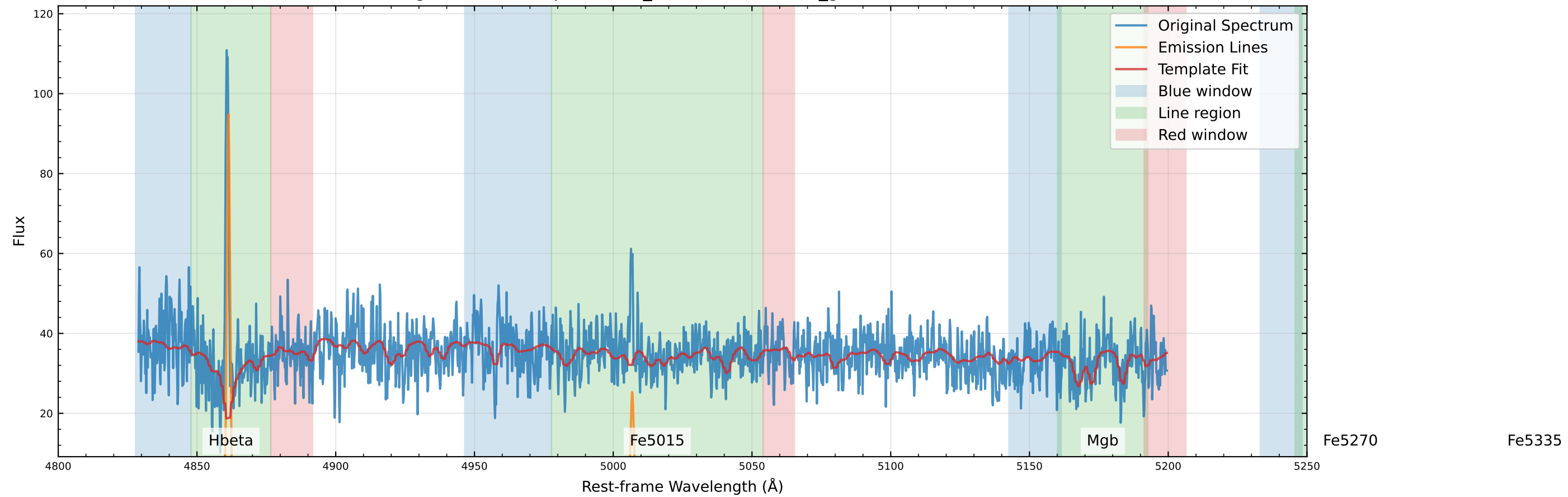
Original Data Comparison (v_star=-44.7 km/s, v_gas=-29.8 km/s)
