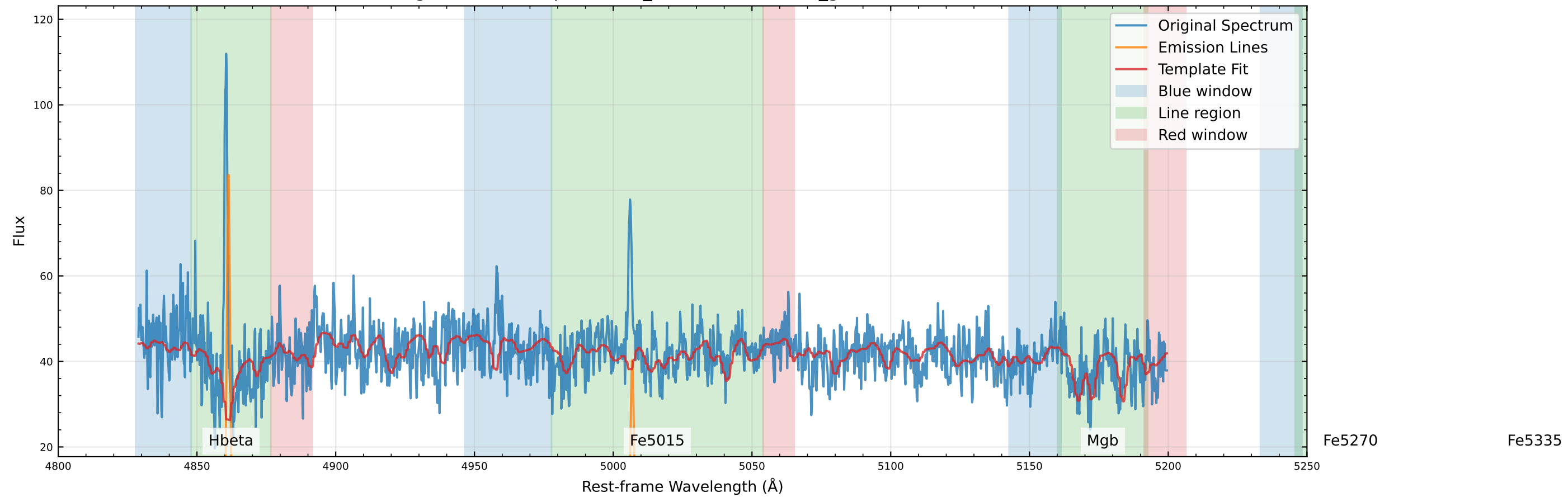
Original Data Comparison (v_star=-71.1 km/s, v_gas=-55.1 km/s)
