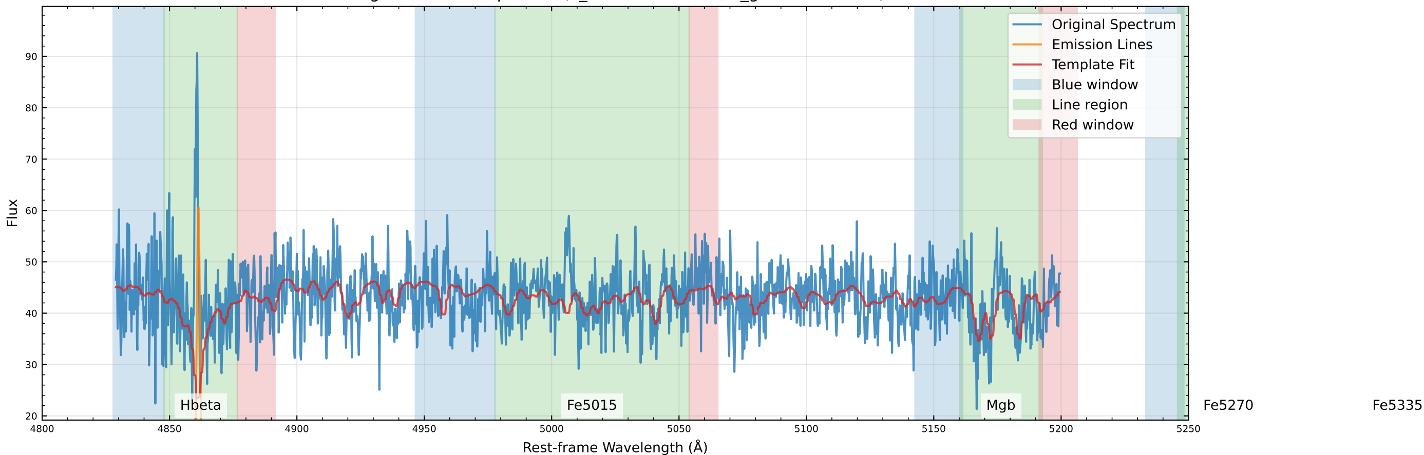
Original Data Comparison (v_star=-48.0 km/s, v_gas=-46.2 km/s)
