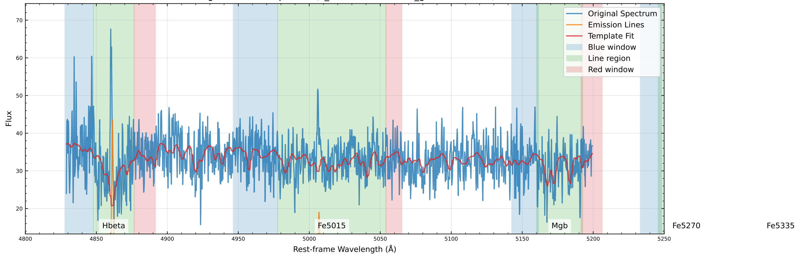
Original Data Comparison ( v_{\text{star}}=-57.3 km/s, v_{\text{gas}}=-54.8 km/s)
