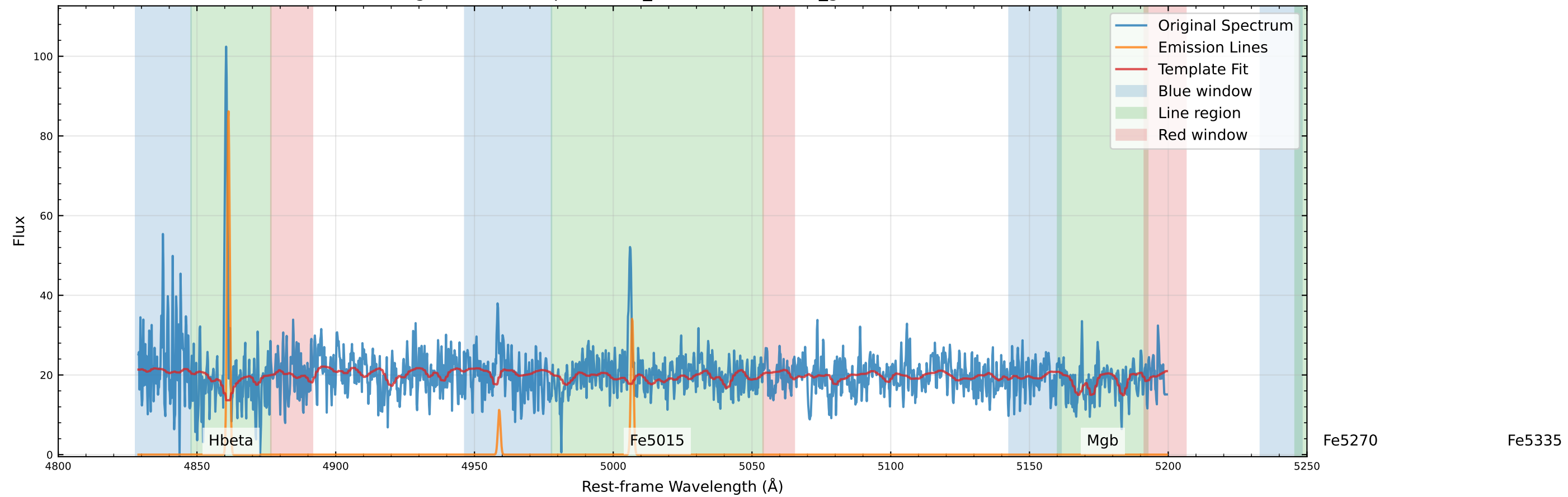
Original Data Comparison (v_star=-86.5 km/s, v_gas=-53.2 km/s)
