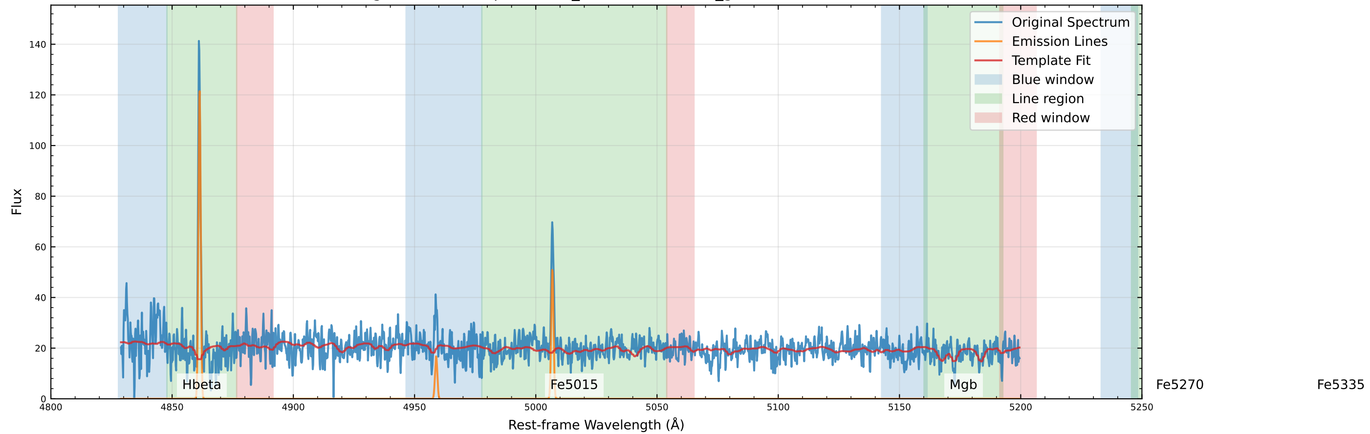
Original Data Comparison (v_star=-6.1 km/s, v_gas=-7.5 km/s)
