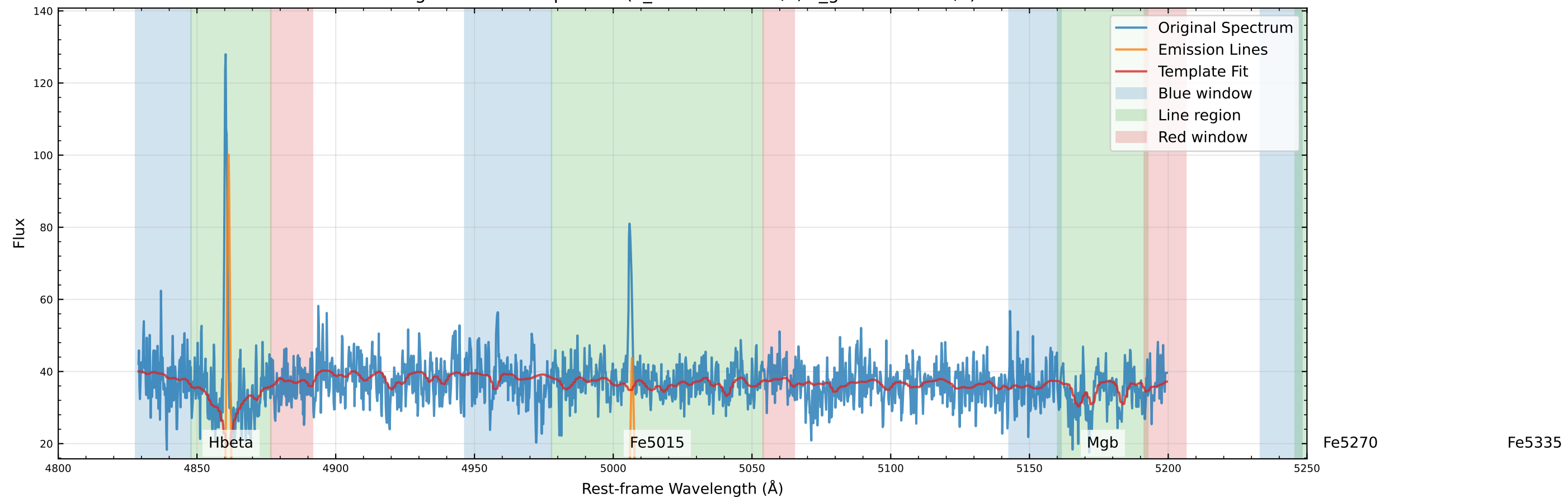
Original Data Comparison (v_star=-67.6 km/s, v_gas=-55.9 km/s)
