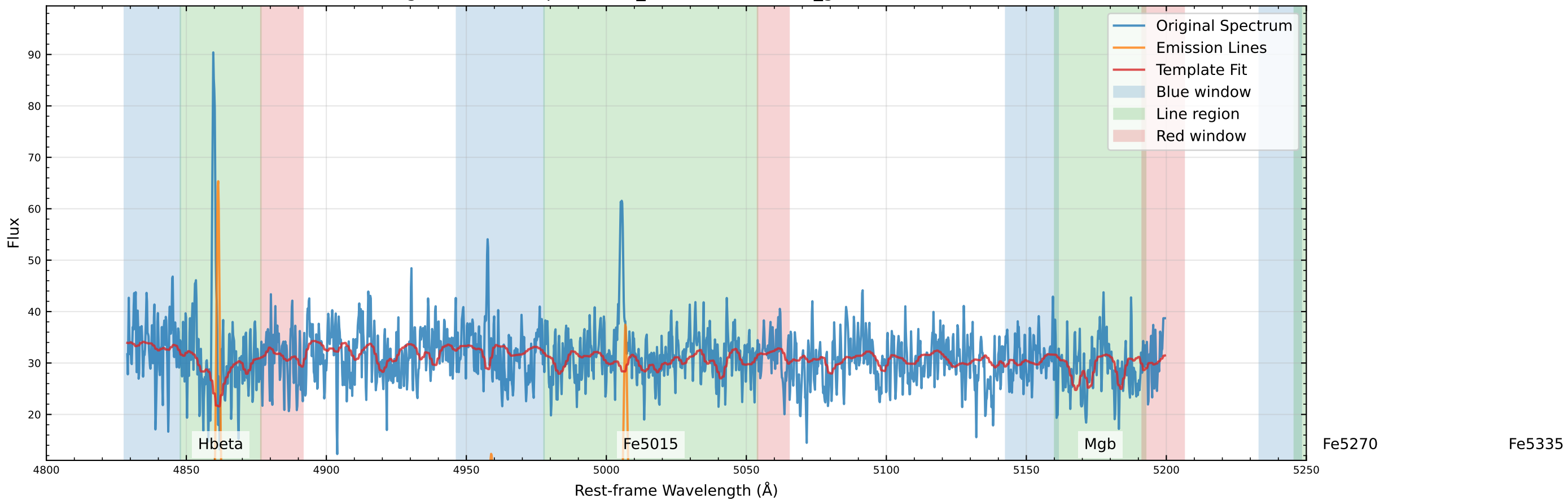
Original Data Comparison (v_star=-77.0 km/s, v_gas=-91.5 km/s)
