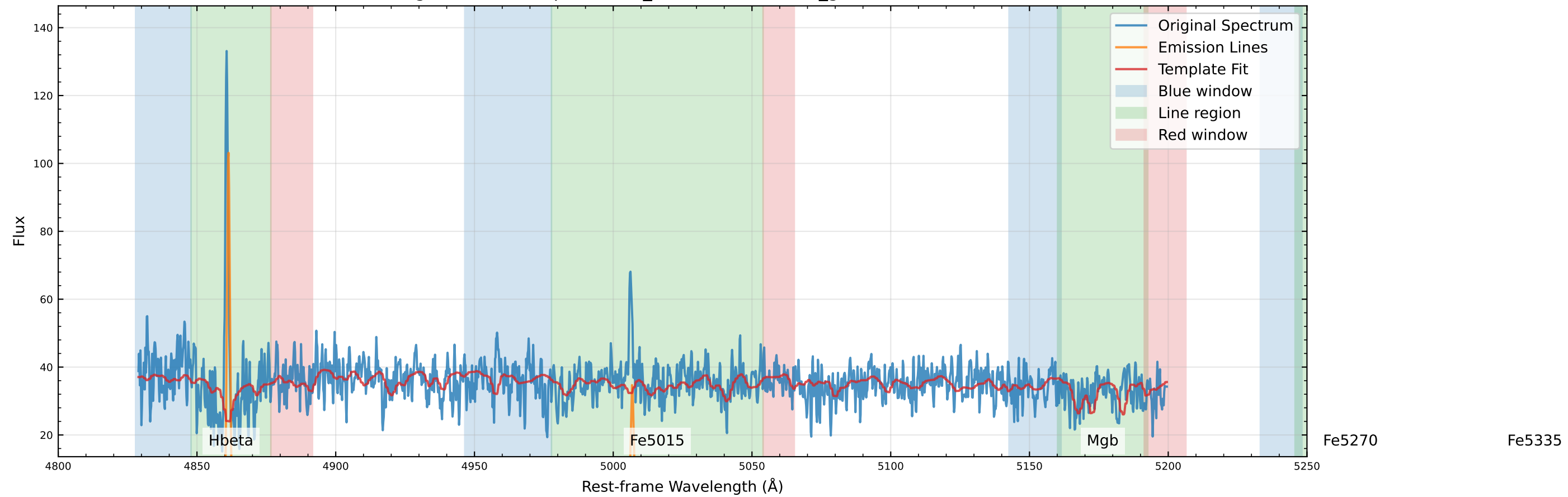
Original Data Comparison (v_star=-78.0 km/s, v_gas=-38.6 km/s)
