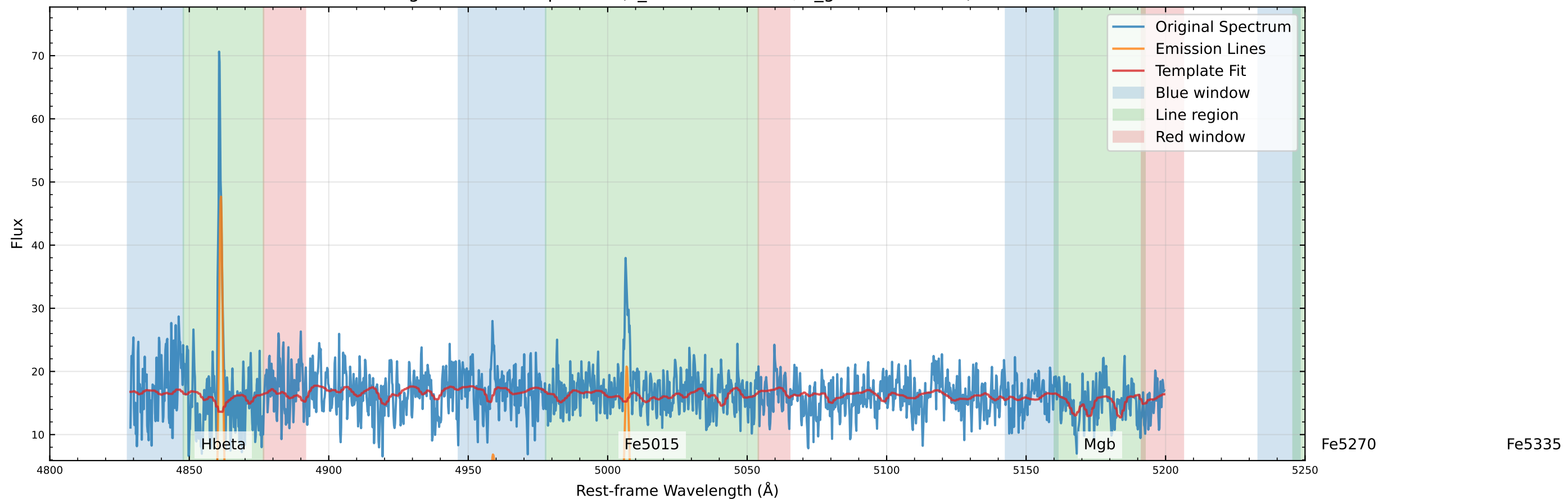
Original Data Comparison ( v_{\text{star}}=-22.4 km/s, v_{\text{gas}}=-19.7 km/s)
