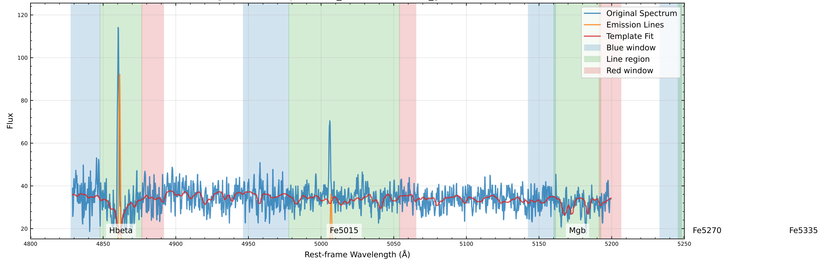
Original Data Comparison (v_star=-94.6 km/s, v_gas=-57.8 km/s)
