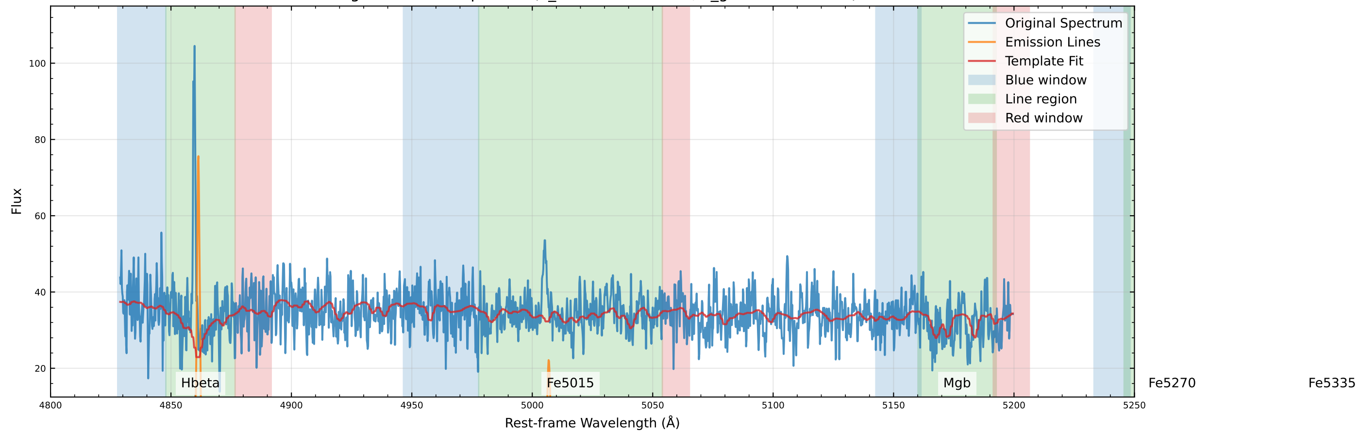
Original Data Comparison (v_star=-104.4 km/s, v_gas=-103.4 km/s)
