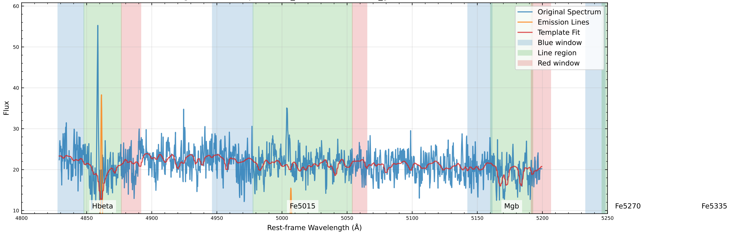
Original Data Comparison (v_star=-165.6 km/s, v_gas=-177.3 km/s)
