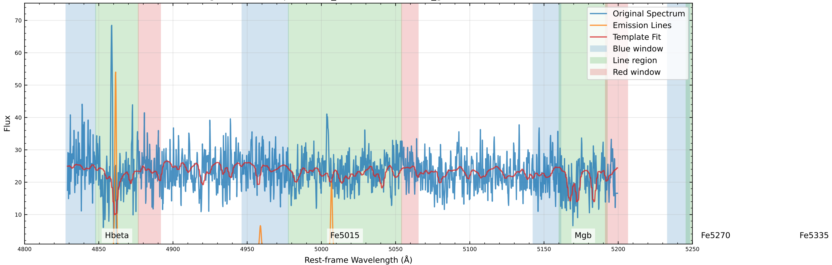
Original Data Comparison (v_star=-175.8 km/s, v_gas=-166.8 km/s)
