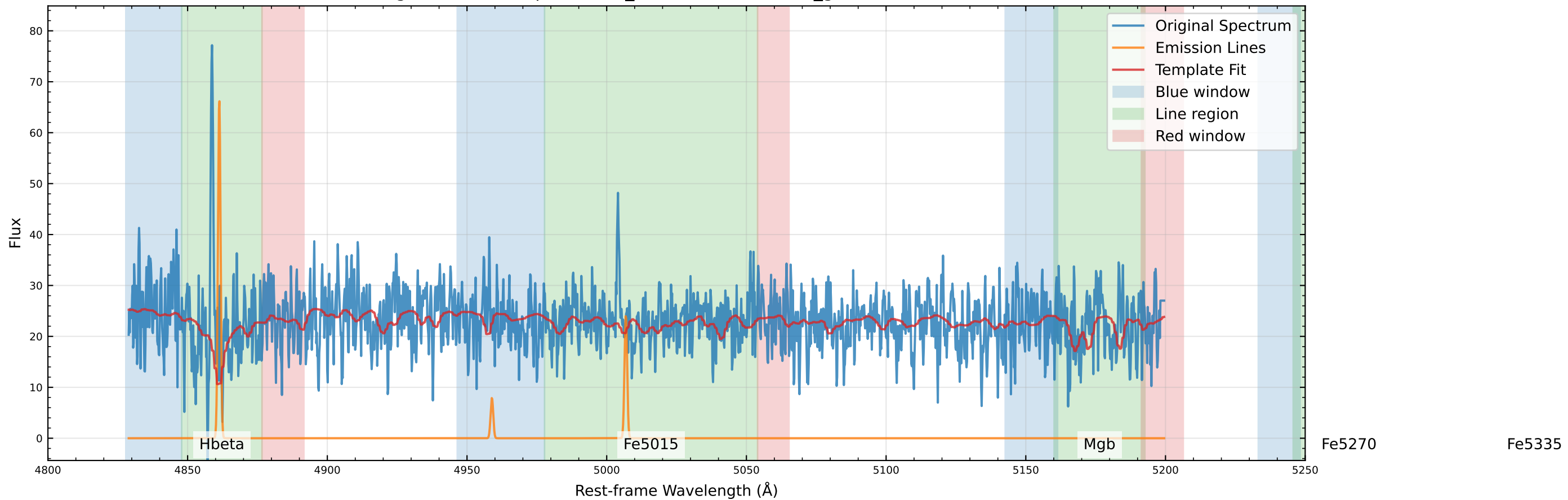
Original Data Comparison ( v_{\text{star}}=-156.6 km/s, v_{\text{gas}}=-162.5 km/s)
