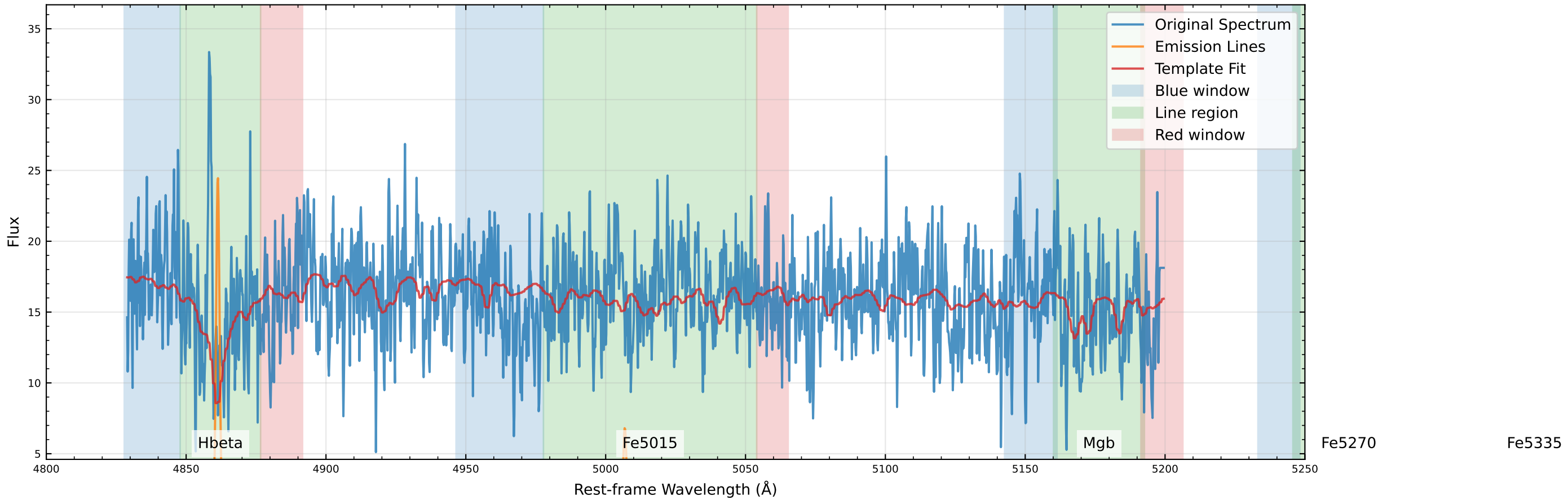
Original Data Comparison (v_star=-176.9 km/s, v_gas=-178.0 km/s)
