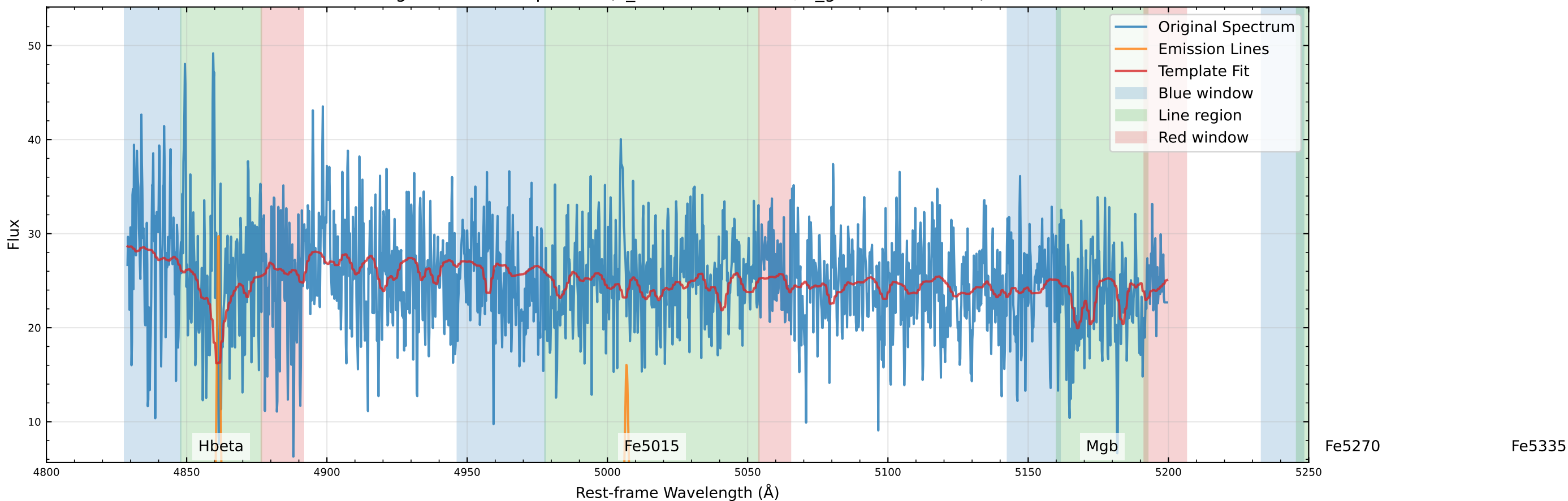
Original Data Comparison (v_star=-111.8 km/s, v_gas=-108.4 km/s)
