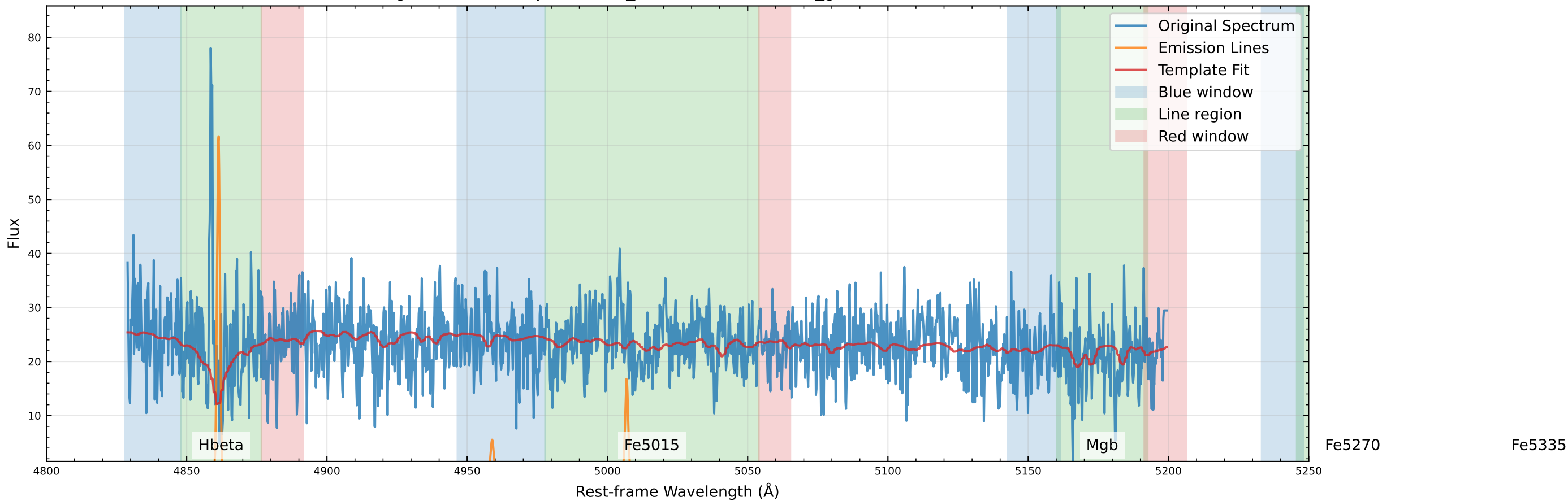
Original Data Comparison (v_star=-152.1 km/s, v_gas=-159.6 km/s)
