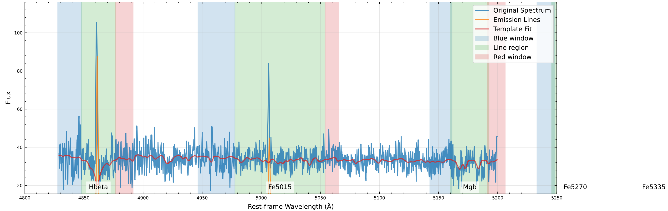
Original Data Comparison (v_star=-35.4 km/s, v_gas=-36.6 km/s)
