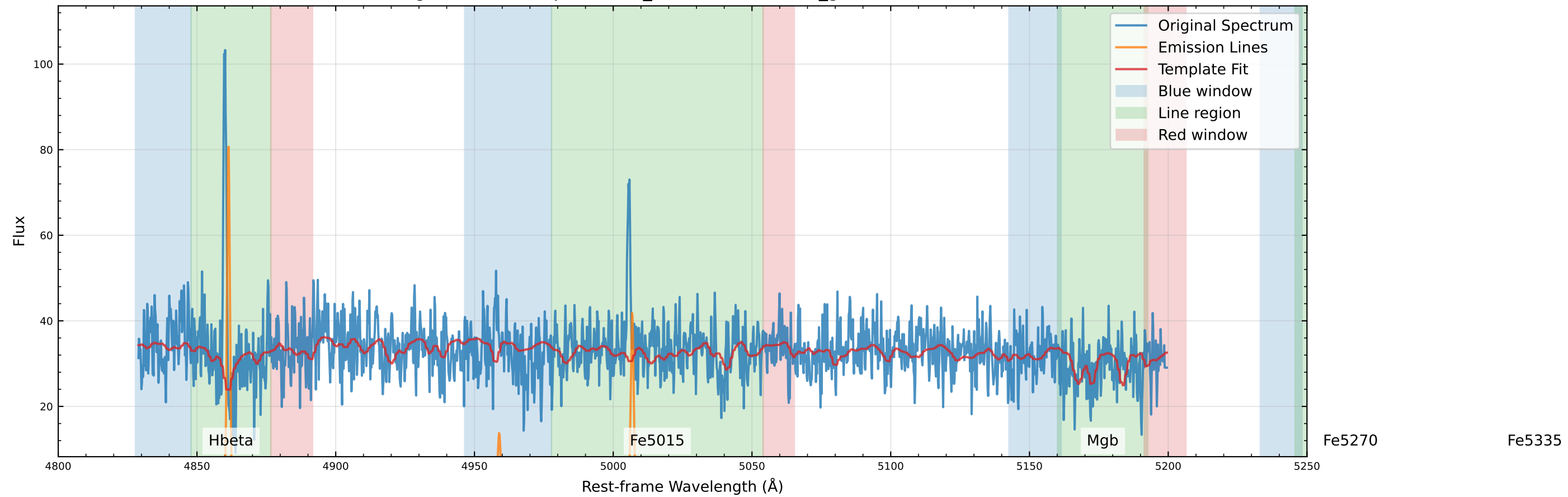
Original Data Comparison (v_star=-87.5 km/s, v_gas=-79.2 km/s)
