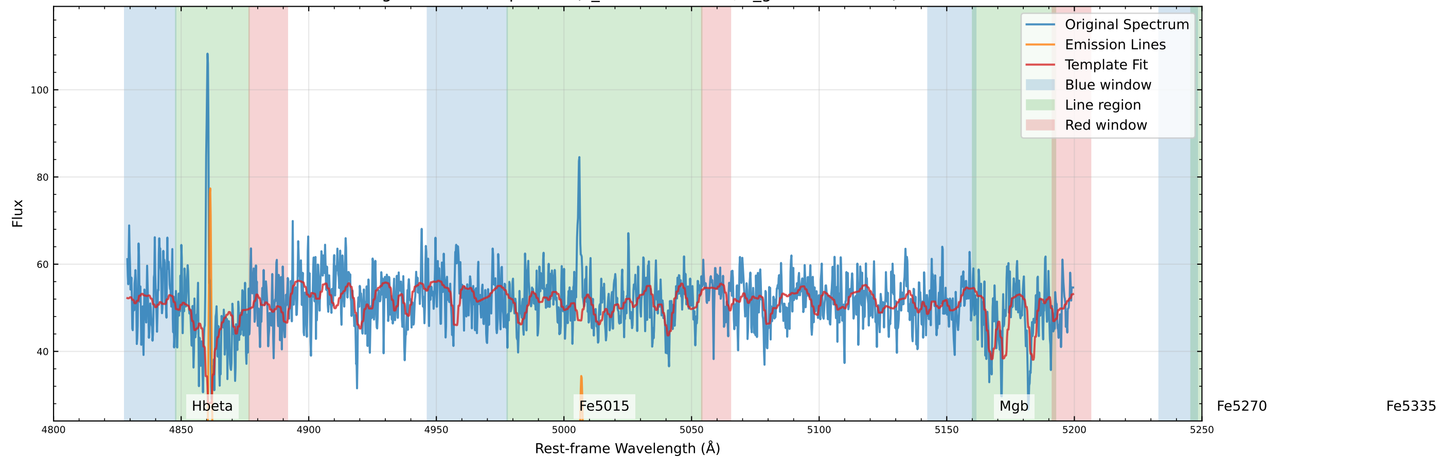
Original Data Comparison (v_star=-67.3 km/s, v_gas=-64.4 km/s)
