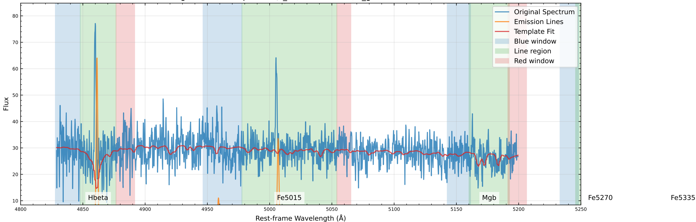
Original Data Comparison (v_star=-71.4 km/s, v_gas=-87.7 km/s)
