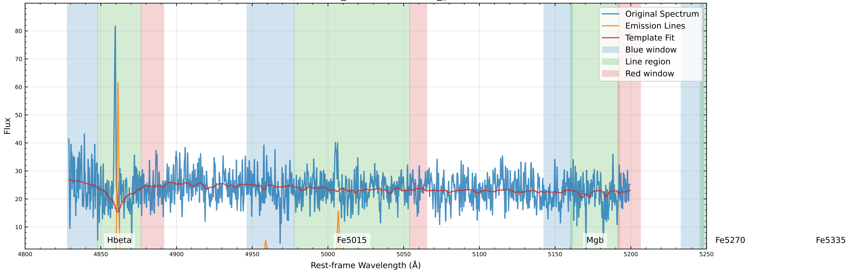
Original Data Comparison (v_star=-82.3 km/s, v_gas=-116.1 km/s)
