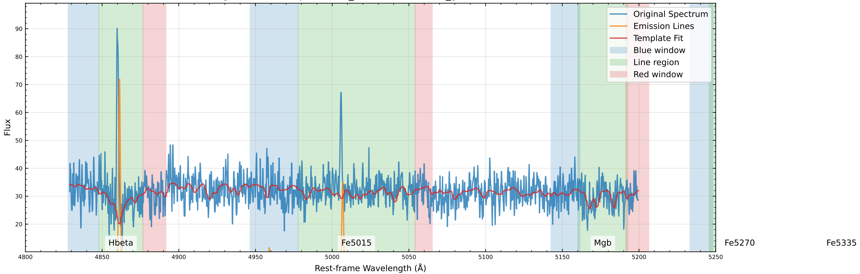
Original Data Comparison (v_star=-82.3 km/s, v_gas=-74.8 km/s)
