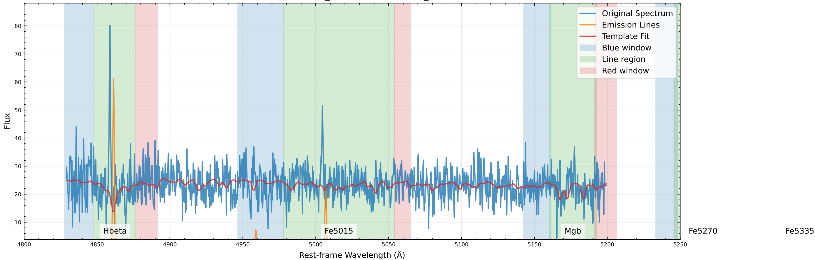
Original Data Comparison (v_star=-146.5 km/s, v_gas=-155.1 km/s)
