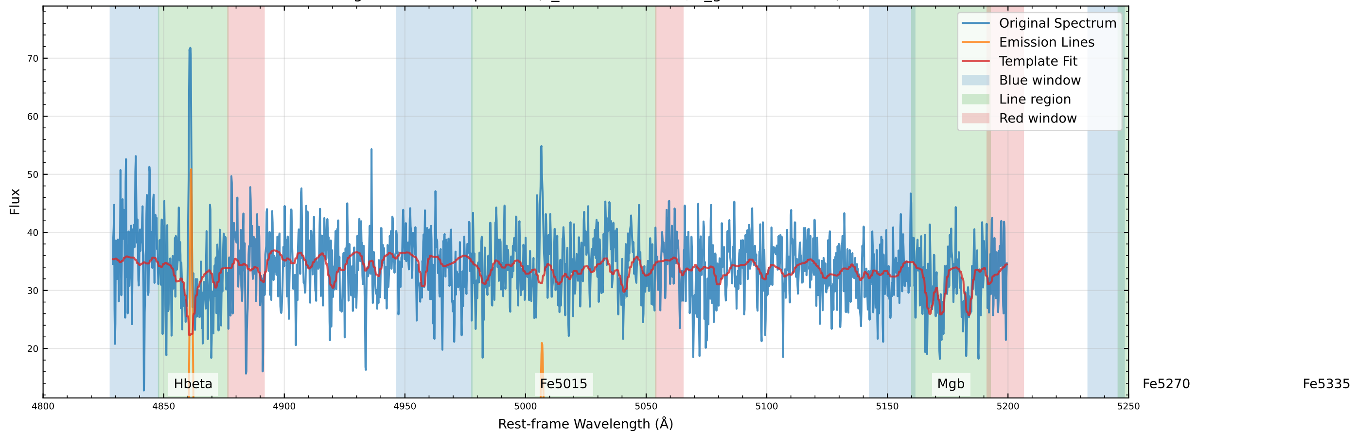
Original Data Comparison (v_star=-19.3 km/s, v_gas=-25.6 km/s)
