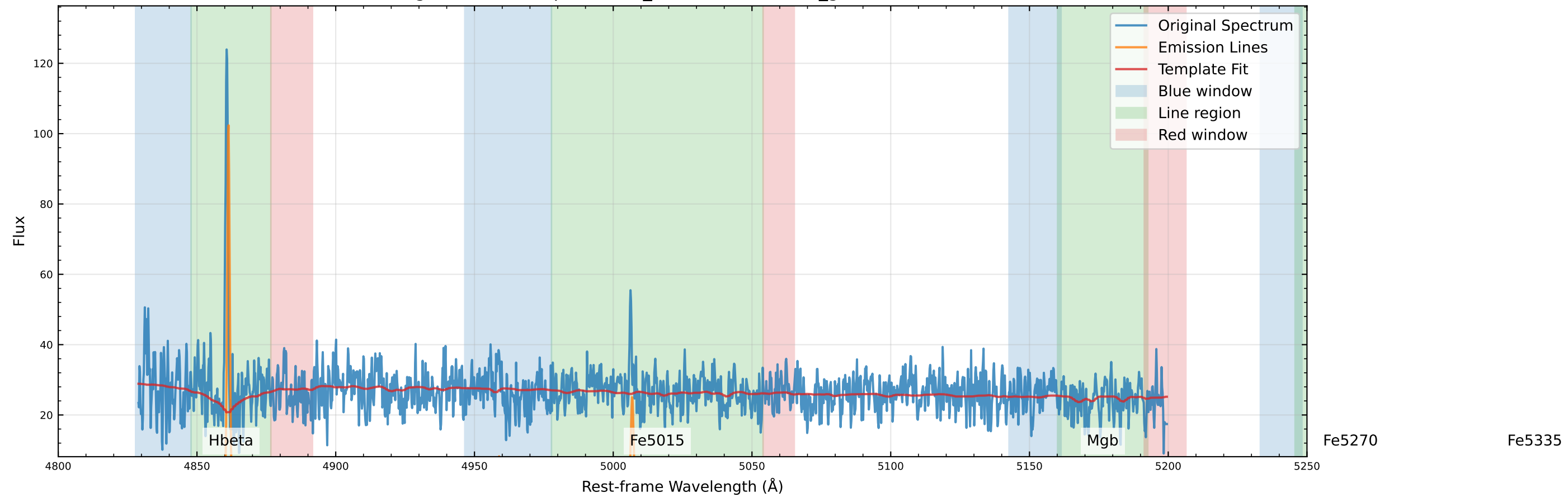
Original Data Comparison (v_star=-76.8 km/s, v_gas=-38.9 km/s)
