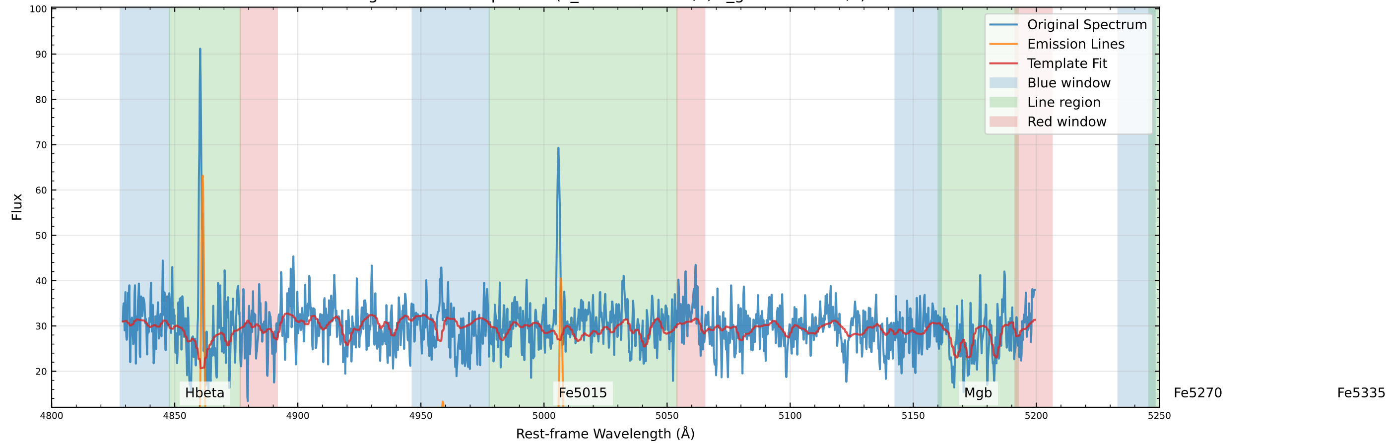
Original Data Comparison (v_star=-55.5 km/s, v_gas=-57.8 km/s)
