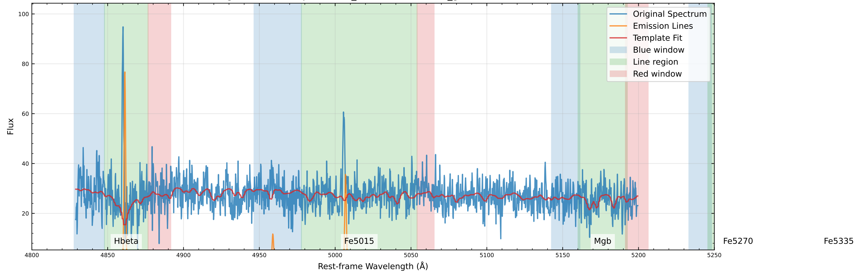
Original Data Comparison (v_star=-67.0 km/s, v_gas=-76.4 km/s)
