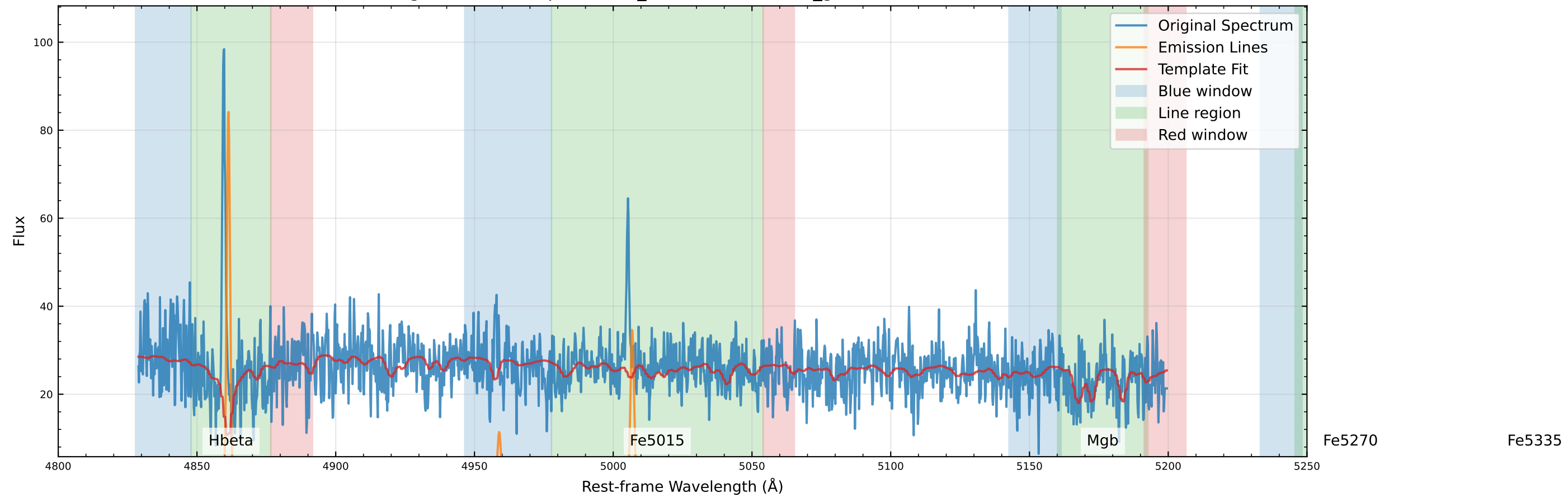
Original Data Comparison (v_star=-84.8 km/s, v_gas=-100.3 km/s)
