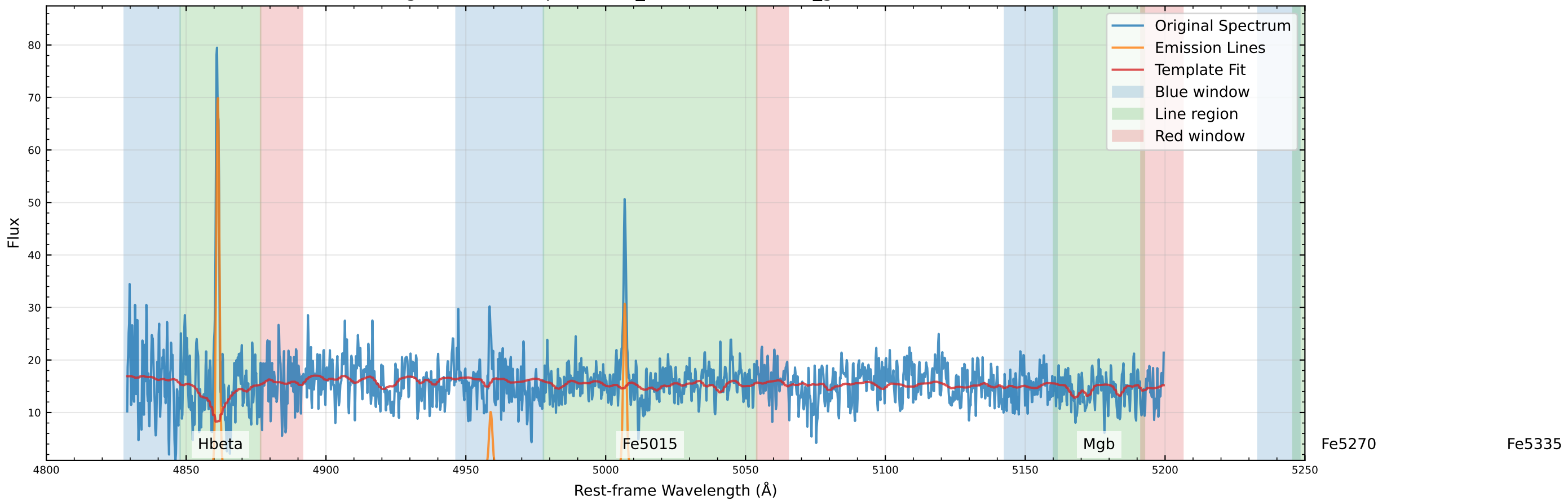
Original Data Comparison (v_star=-22.4 km/s, v_gas=-10.9 km/s)
