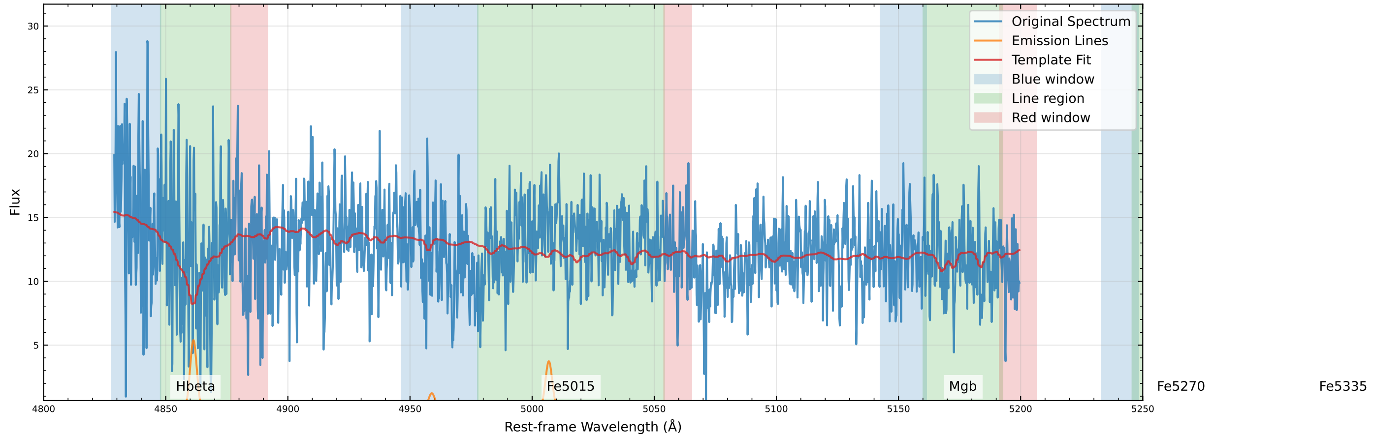
Original Data Comparison (v_star=33.5 km/s, v_gas=-34.7 km/s)
