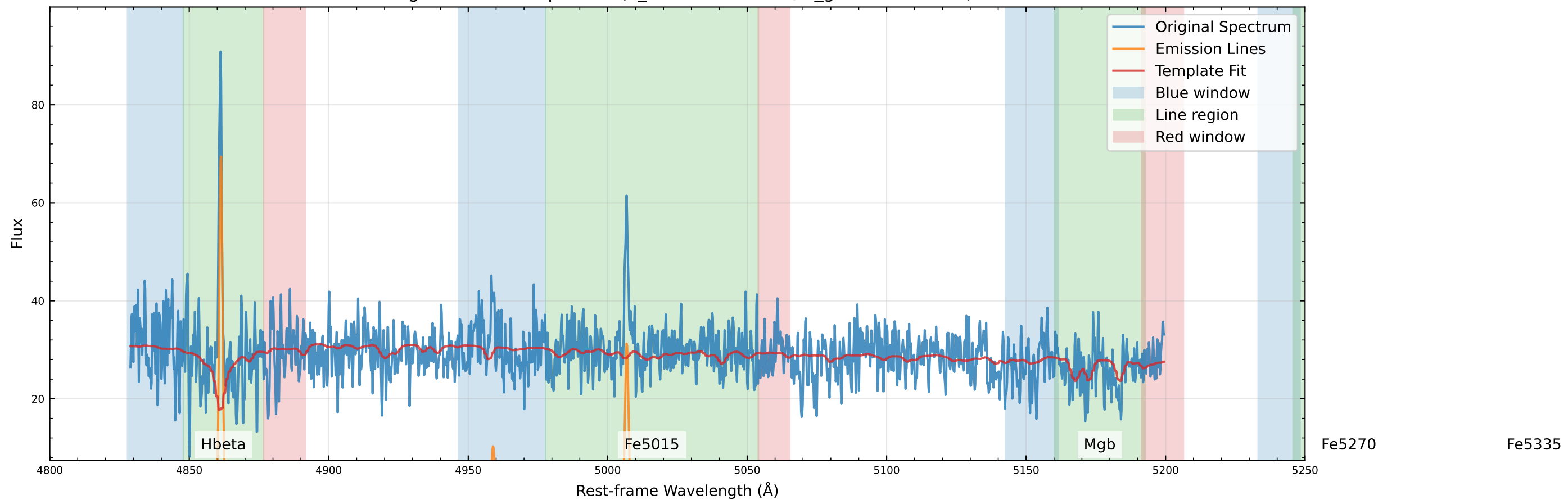
Original Data Comparison ( v_{\text{star}}=-34.3 km/s, v_{\text{gas}}=-12.6 km/s)
