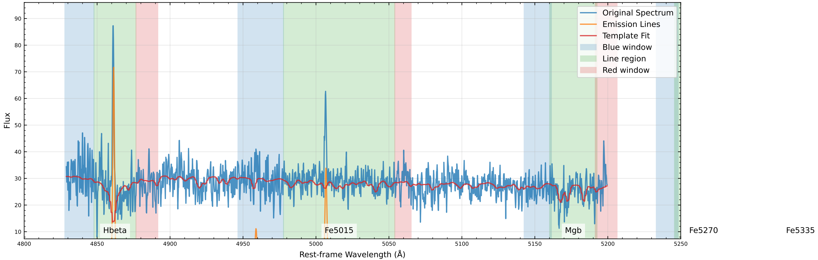
Original Data Comparison (v_star=-34.5 km/s, v_gas=-20.1 km/s)
