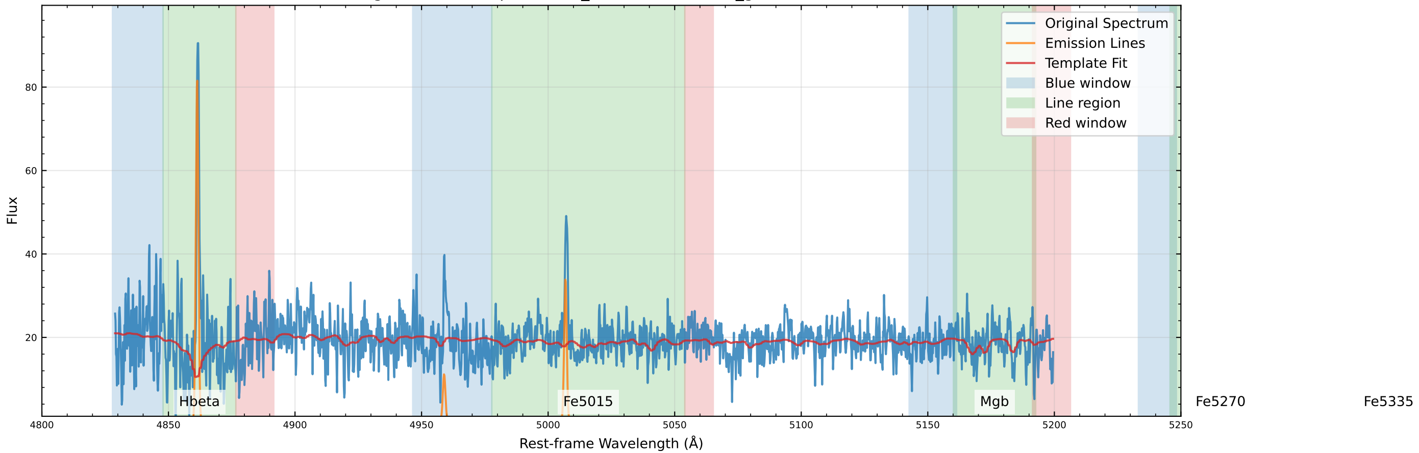
Original Data Comparison (v_star=33.5 km/s, v_gas=20.1 km/s)
