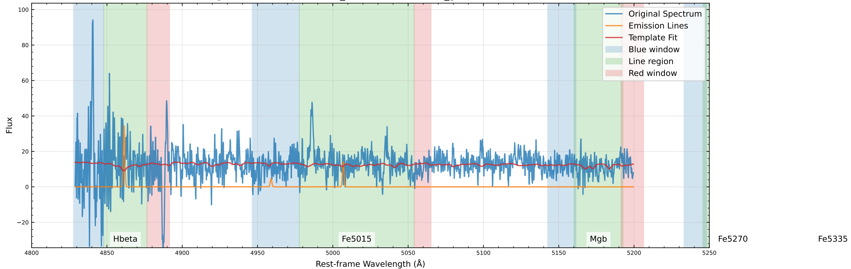
Original Data Comparison (v_star=1838.8 km/s, v_gas=1742.7 km/s)
