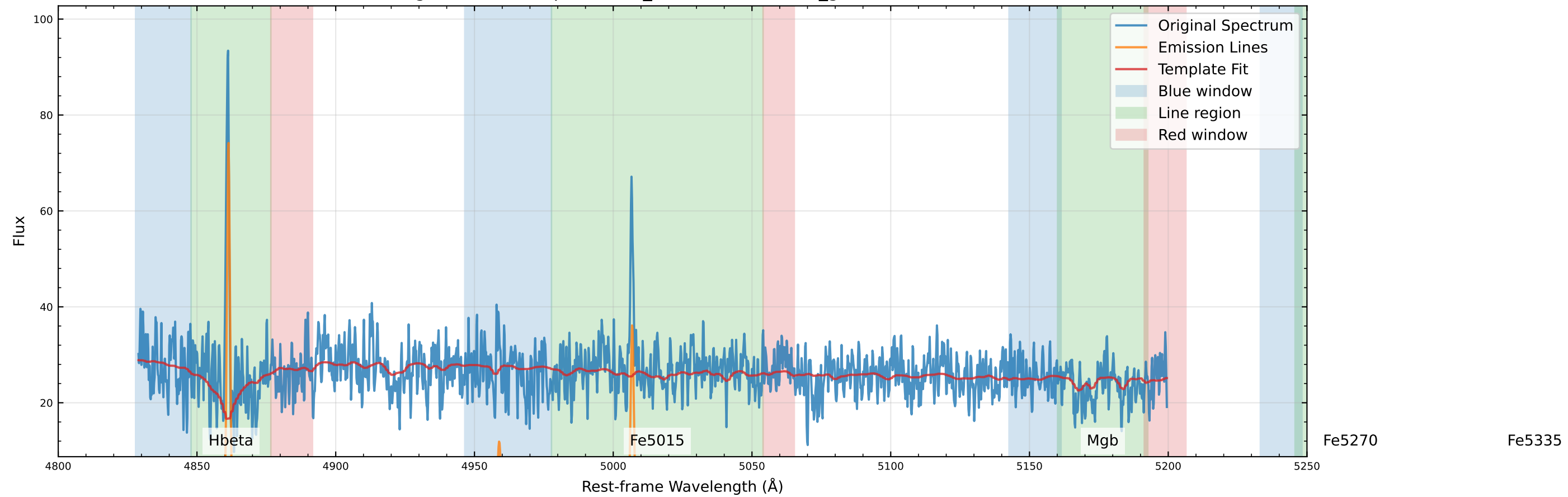
Original Data Comparison (v_star=-11.3 km/s, v_gas=-18.8 km/s)
