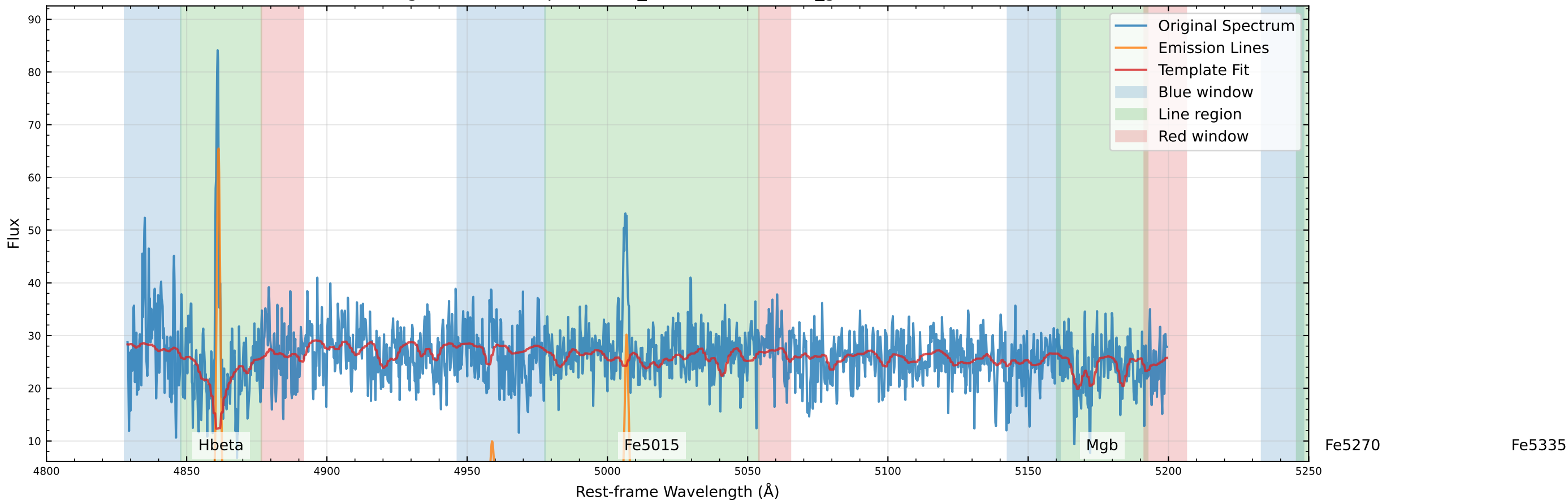
Original Data Comparison (v_star=-44.0 km/s, v_gas=-25.3 km/s)
