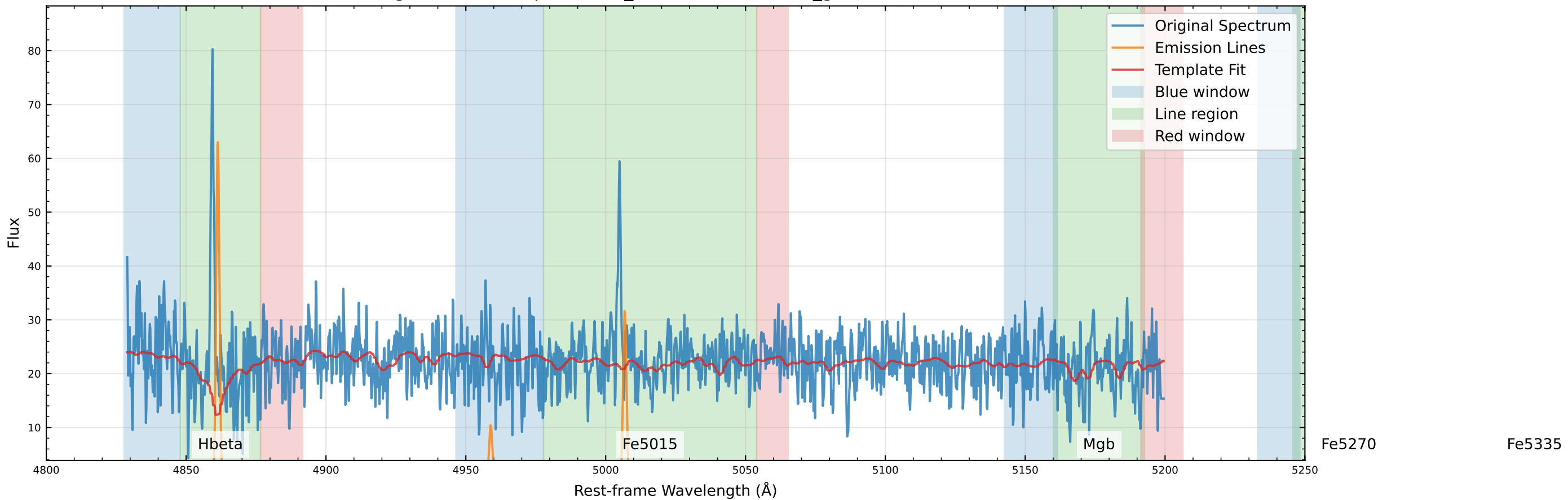
Original Data Comparison (v_star=-114.4 km/s, v_gas=-120.7 km/s)
