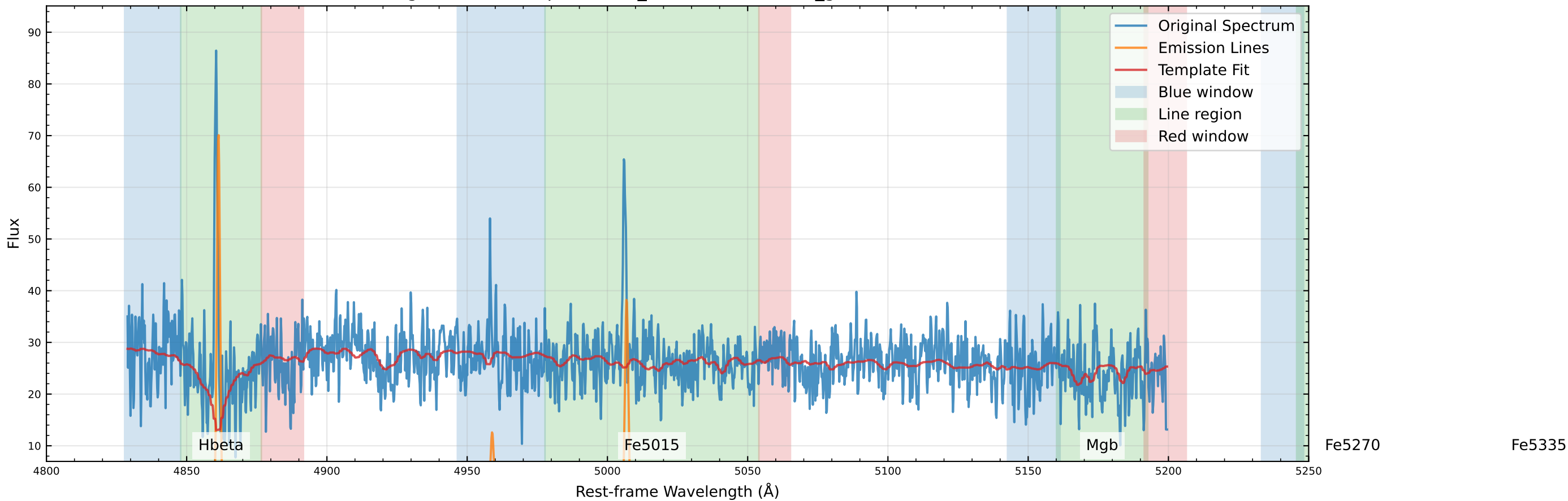
Original Data Comparison (v_star=-48.9 km/s, v_gas=-51.7 km/s)
