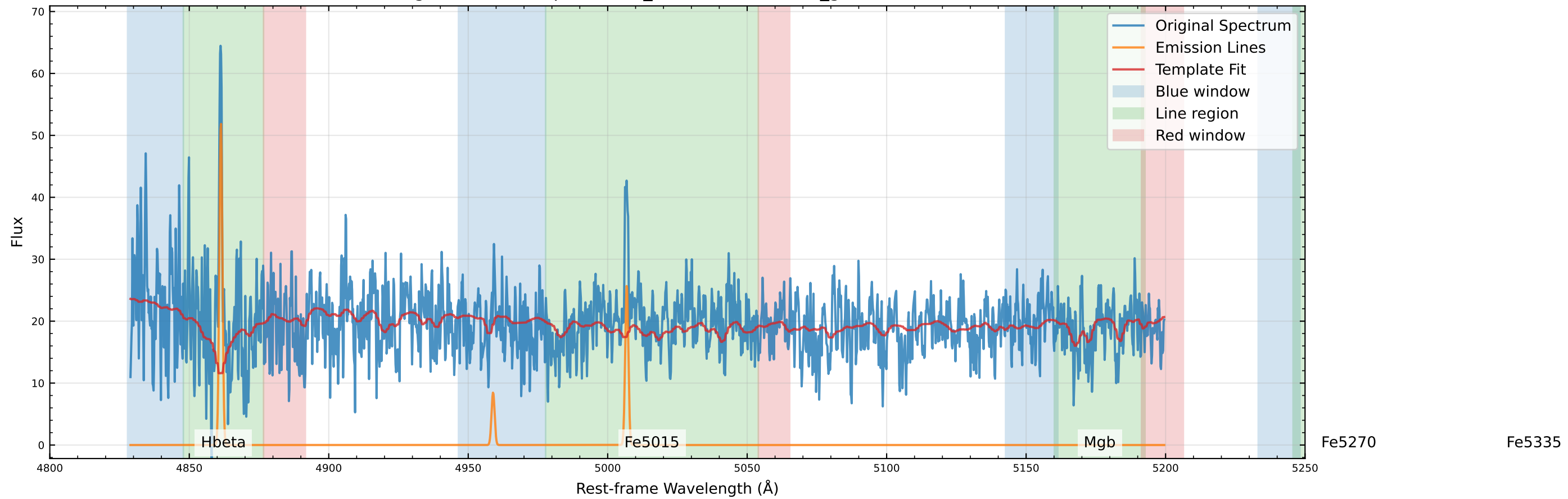
Original Data Comparison (v_star=-22.8 km/s, v_gas=-7.9 km/s)
