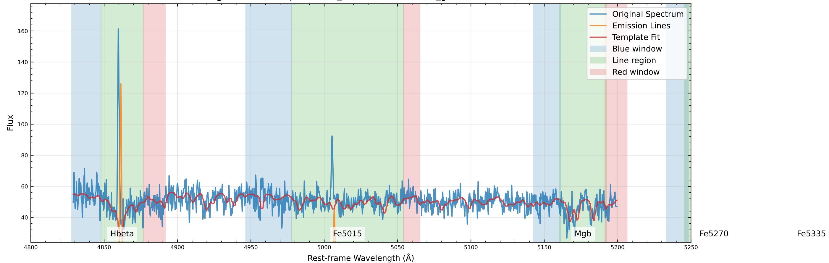
Original Data Comparison (v_star=-101.9 km/s, v_gas=-96.3 km/s)
