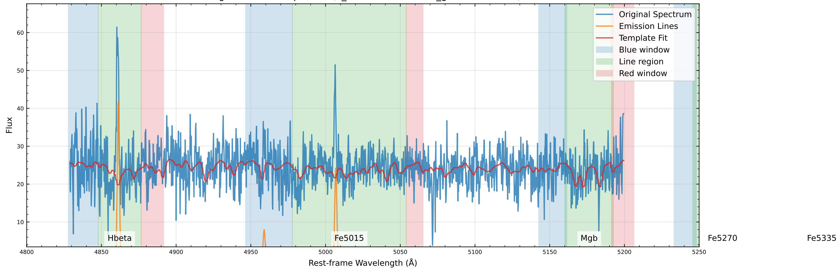
Original Data Comparison (v_star=-59.0 km/s, v_gas=-33.3 km/s)
