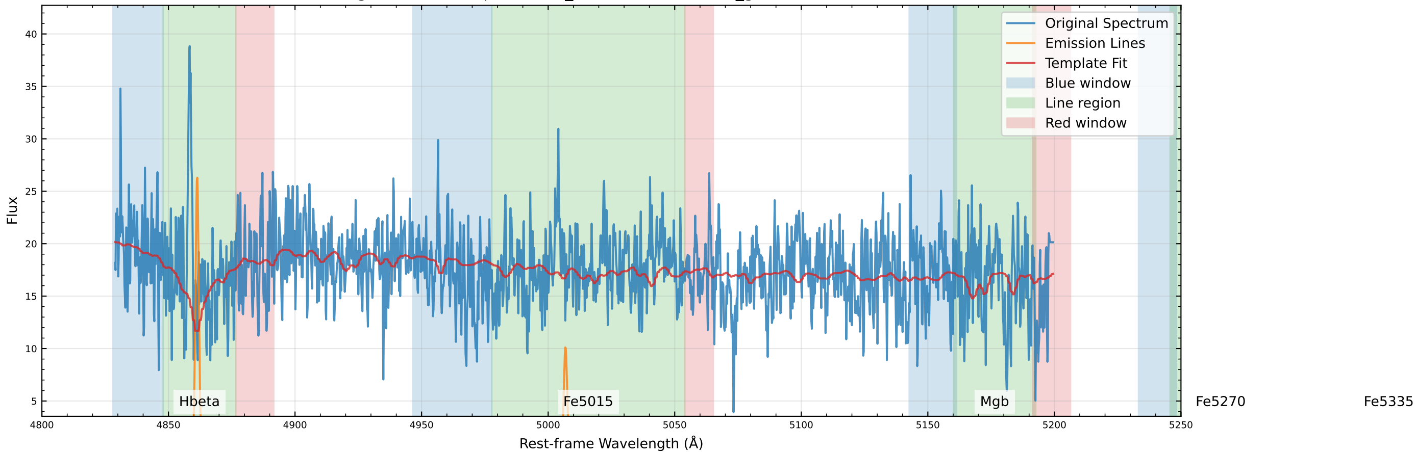
Original Data Comparison (v_star=-172.8 km/s, v_gas=-176.8 km/s)
