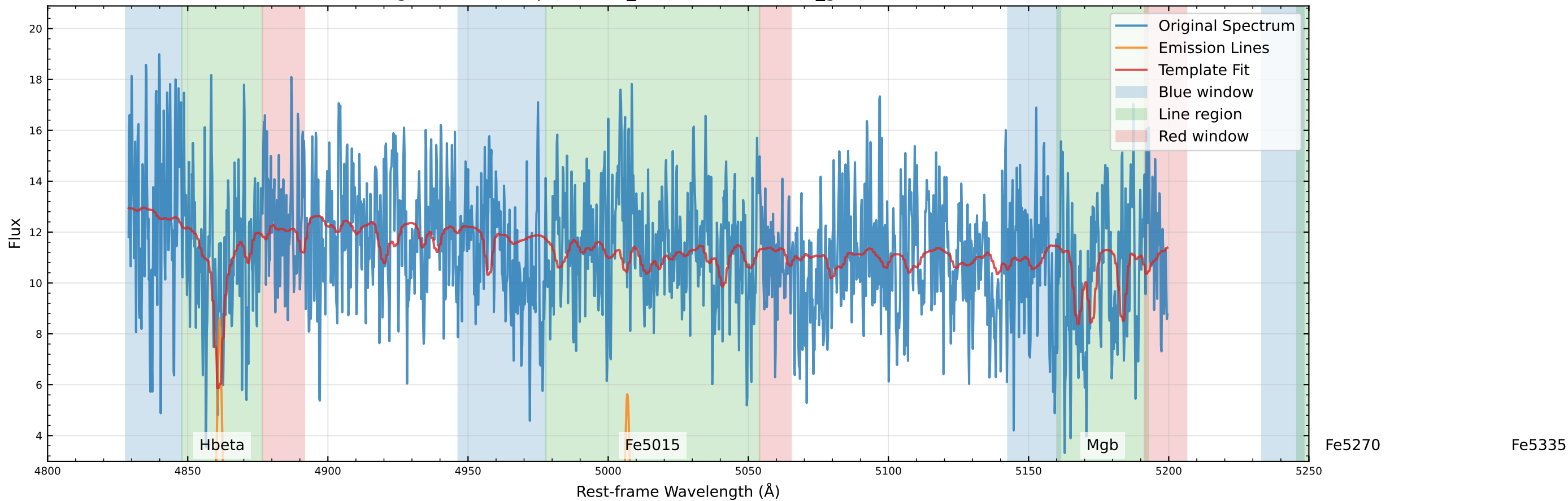
Original Data Comparison (v_star=-180.2 km/s, v_gas=-182.0 km/s)
