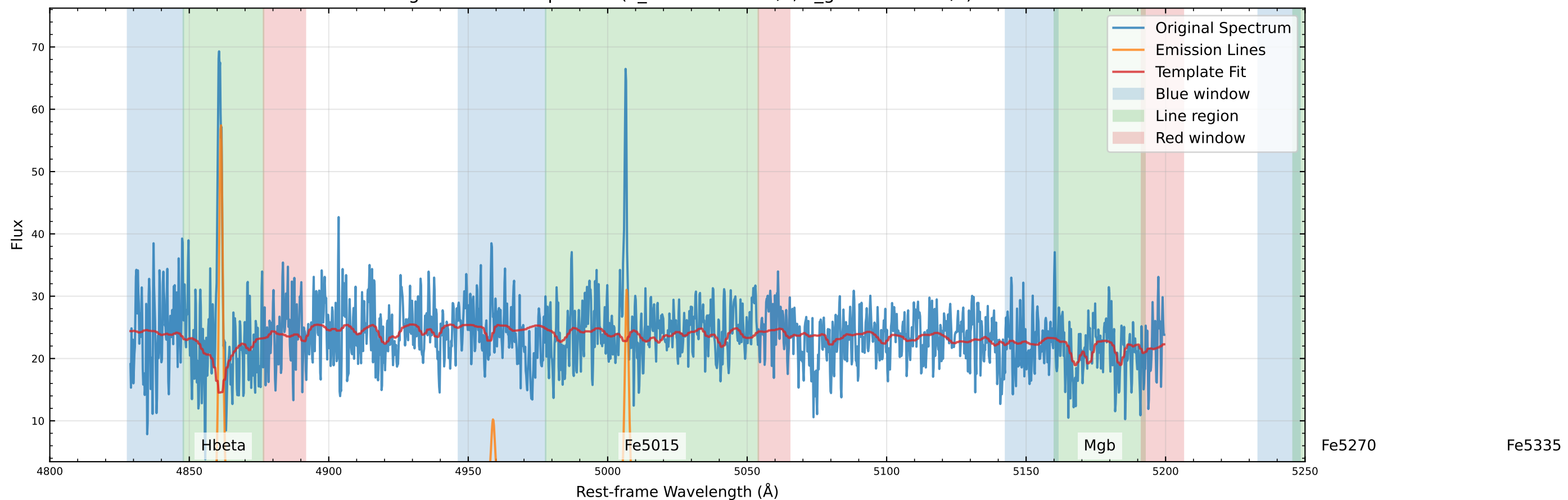
Original Data Comparison ( v_{\text{star}}=-38.1 km/s, v_{\text{gas}}=-29.9 km/s)
